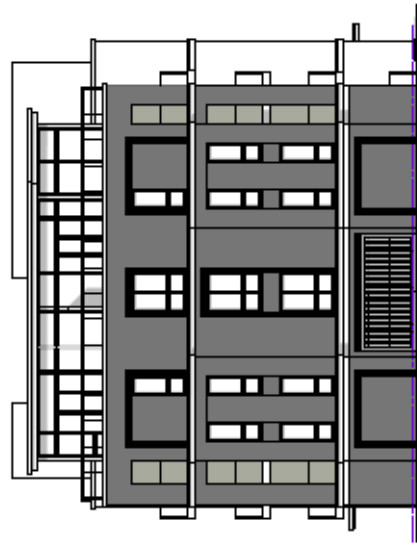
Side Elevation (South) Building H (Plan 205-230)
