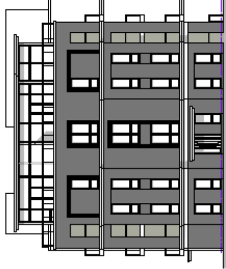
Side Elevation (West) Building C (Plans 3A-3D)
